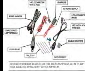
Nighthawk driving lamp wiring loom kit
